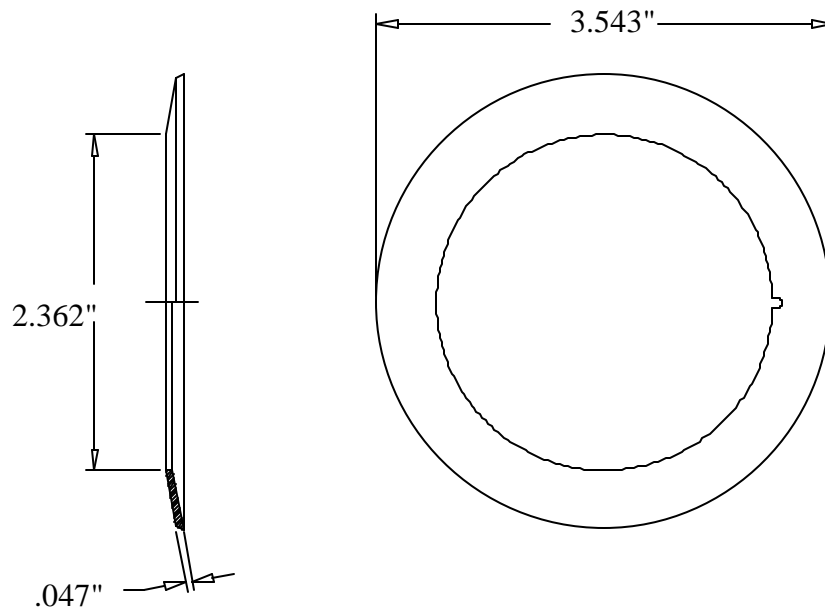
Dished Slitter Knife PART #30601
